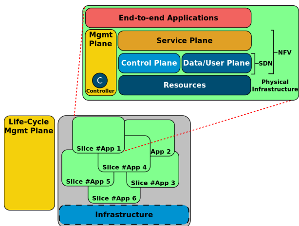
Fig. 3 5G slice template and instantiated slices on top of a common infrastructure.
