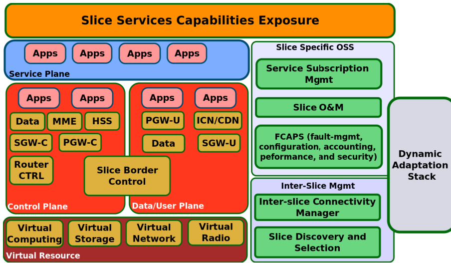
Fig. 5 Slice high-level architecture.
