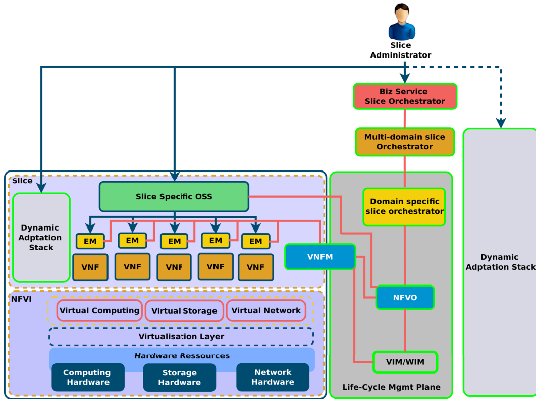
Fig. 6 Orchestration architecture.
