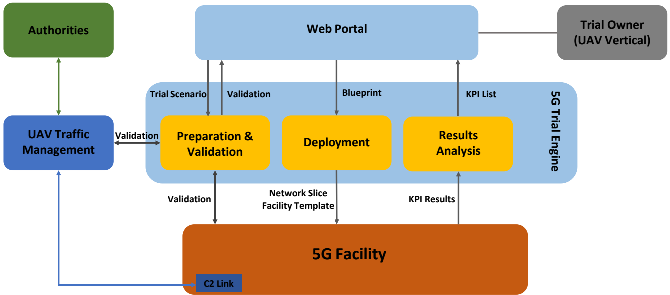
Fig. 2. 5G!Drones UAV trial architecture
